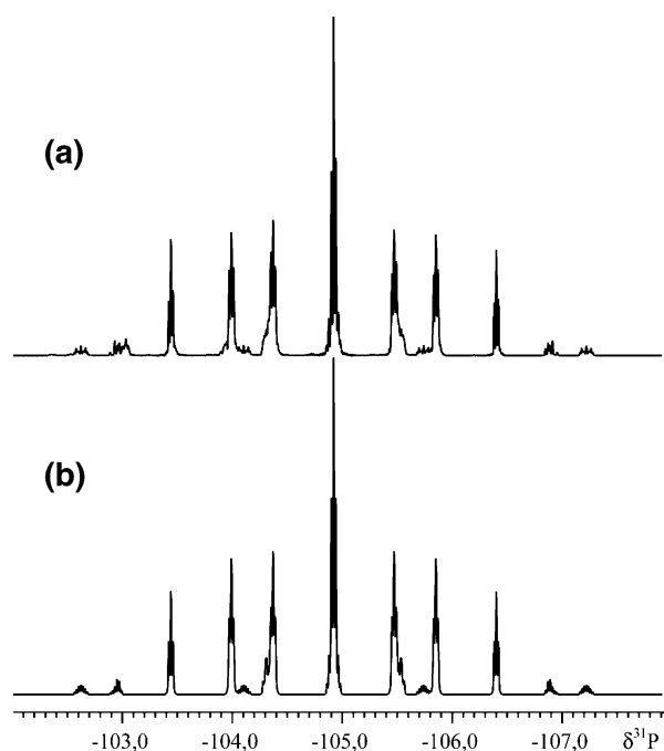
Figure 1. 31 P NMR spectrum of compound 9 . (a) Experimental spectrum (in CD 2 Cl 2 at 25 °C) and (b) calculated spectrum. (For details, see Table 1.)
